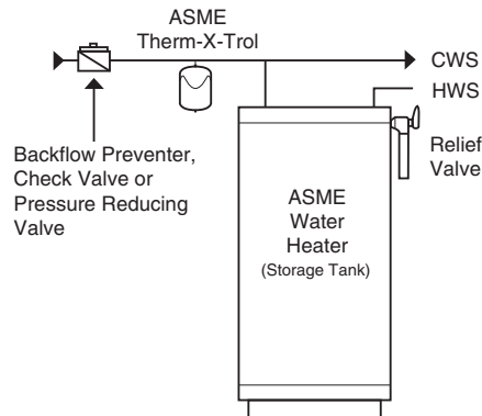
In-Line Installation
